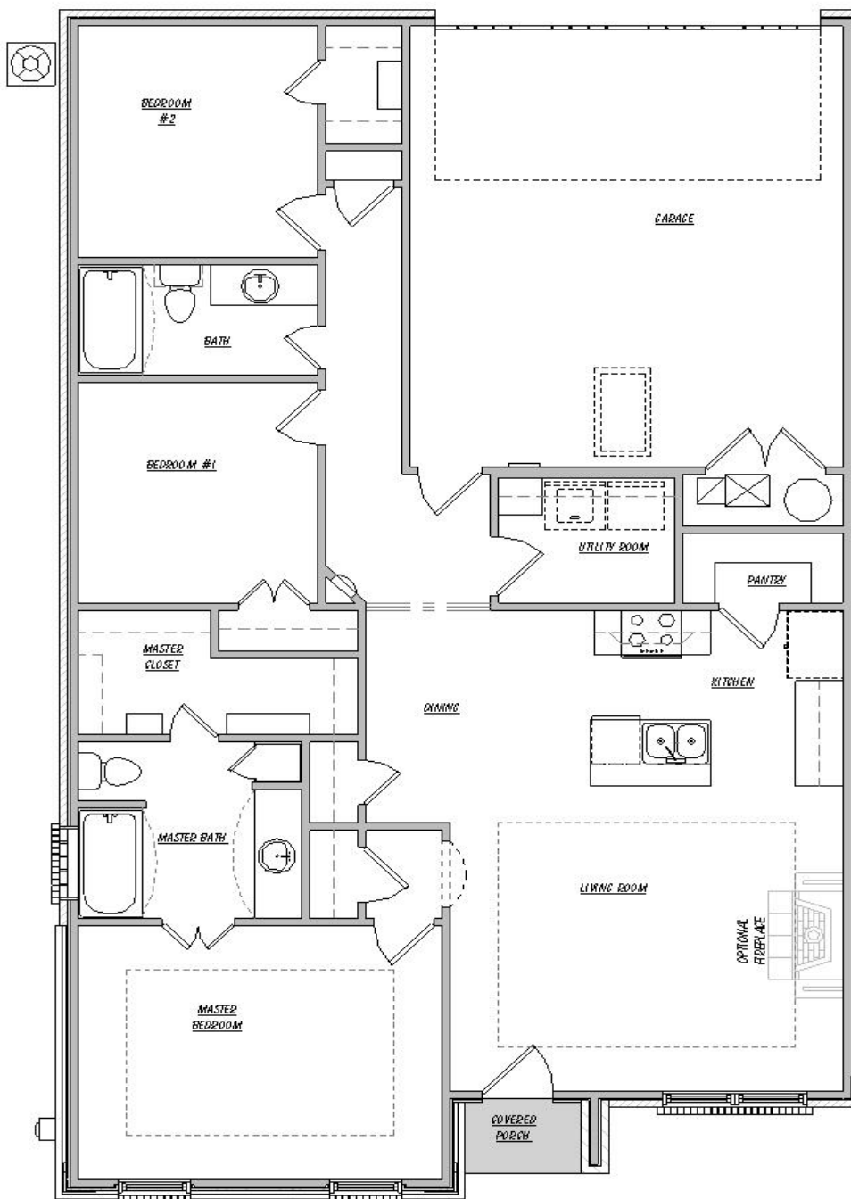
1291A Floor Plan Shown
